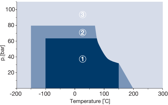
P-T Diagram - thickness 2.0 mm
